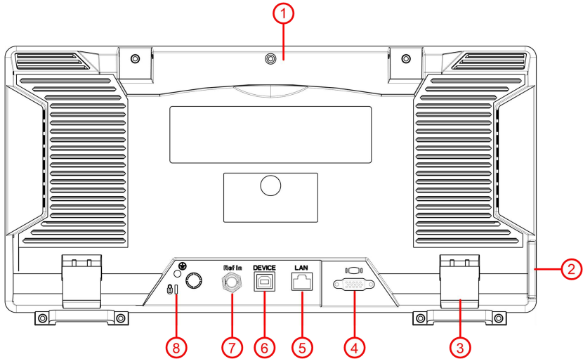
Figure 3-6 Rear Panel
