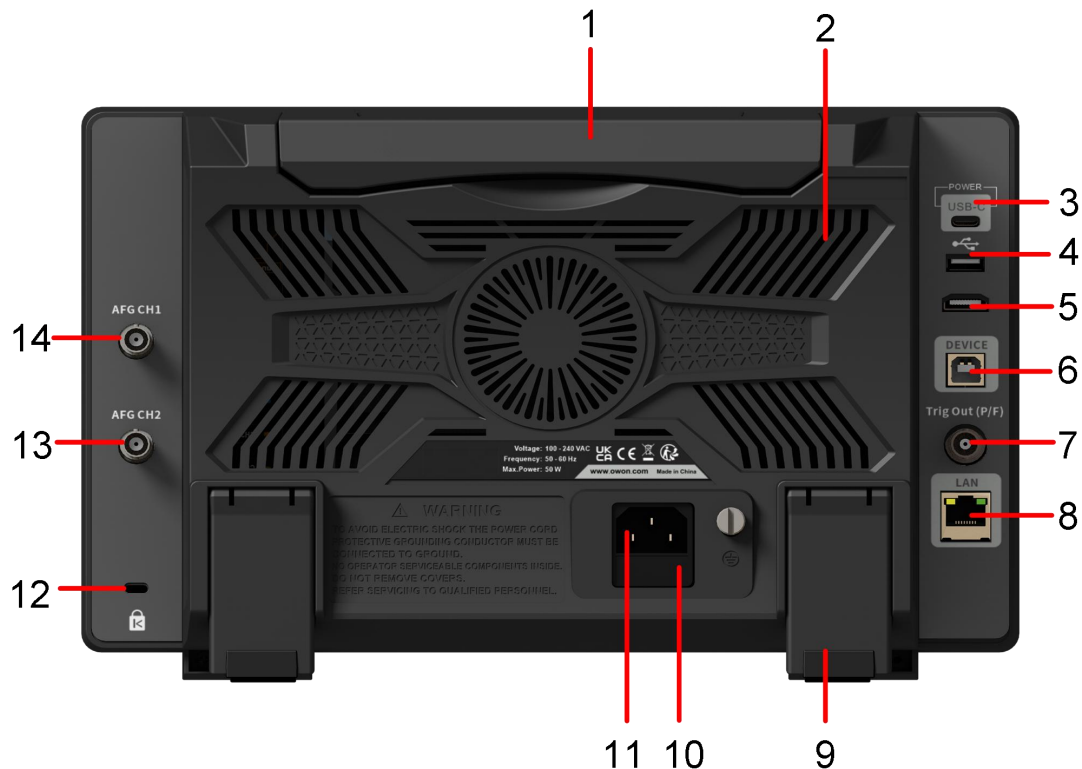
Figure 3-2: Rear Panel
