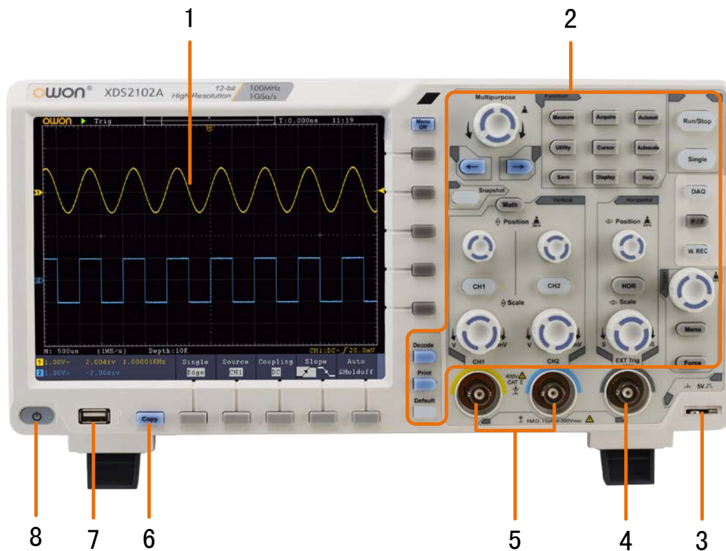
Figure 3-1 Front panel
